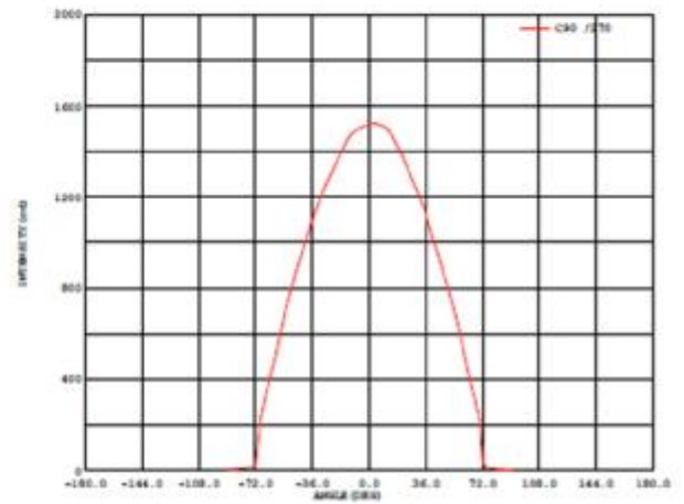
LUMINOUS INTENSITY DISTRIBUTION DIAGRAM
